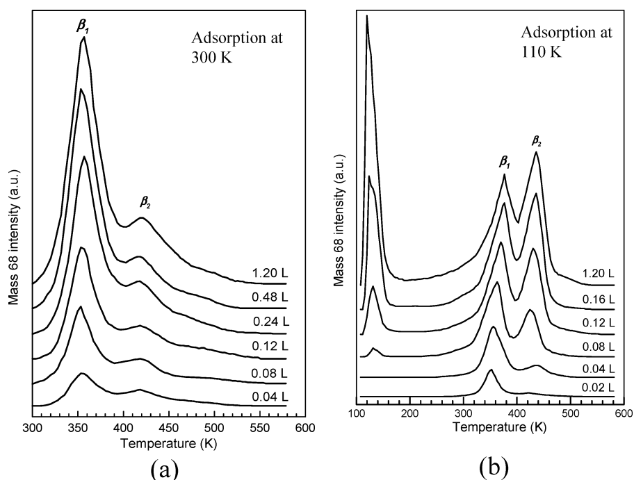
FIGURE 7. TPD spectra of furan ( m/z = 68 ) as a function of the furan exposure at 300 K (a) and at 110 K (b).
